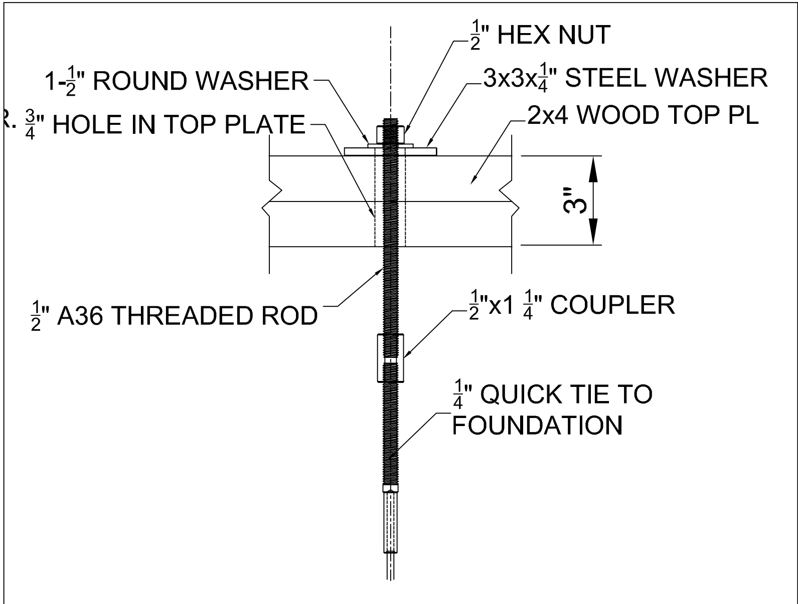
QT - EXTENSION TOP PLATE CONNECTION
